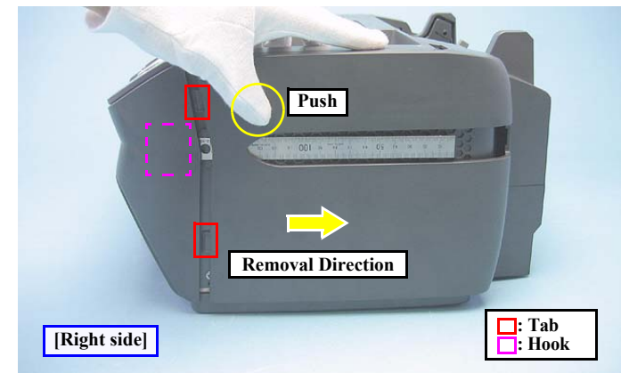
Figure 4-17. Removing the Right/Left Housings (2)
