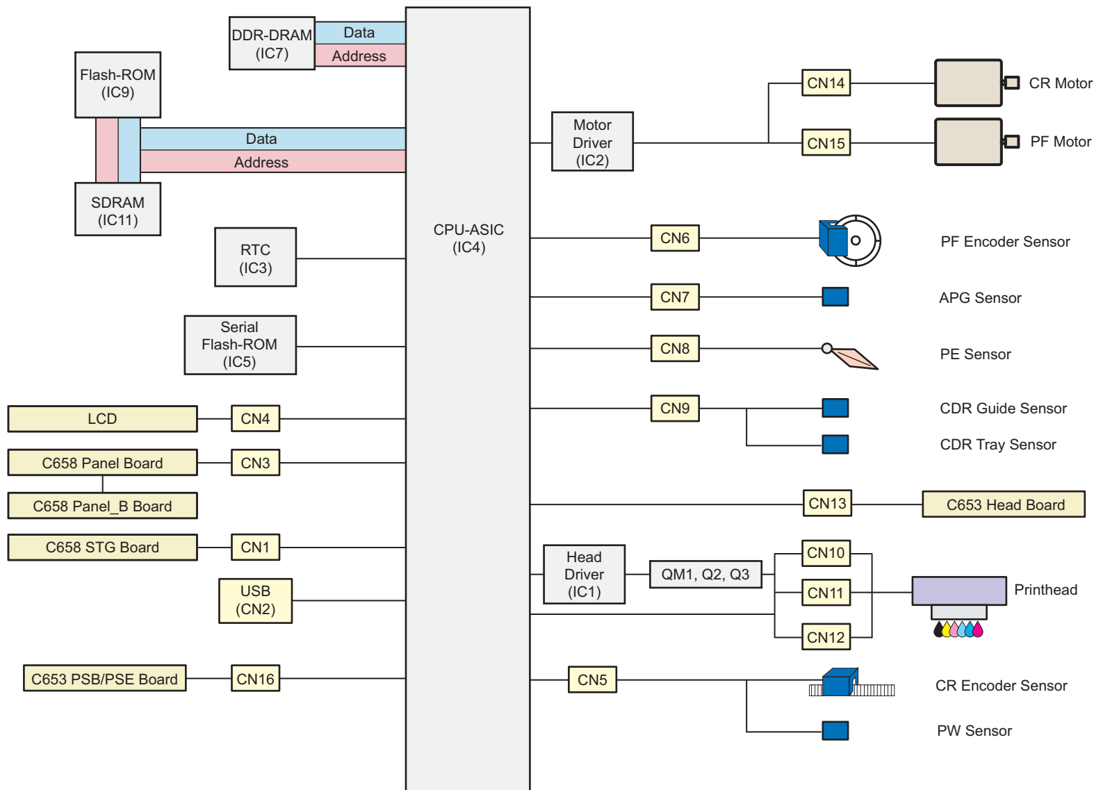
Figure 2-3. Circuit Block Diagram for R360/R380/R390
