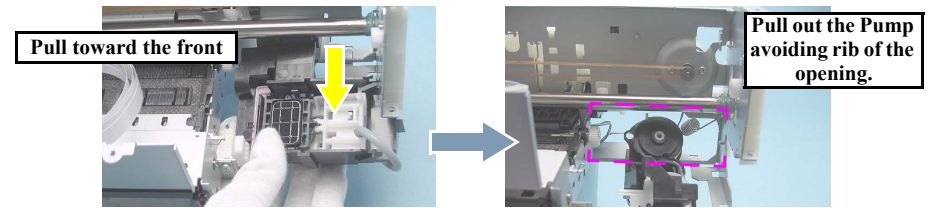
Figure 4-118. Removing the Ink System (2)
