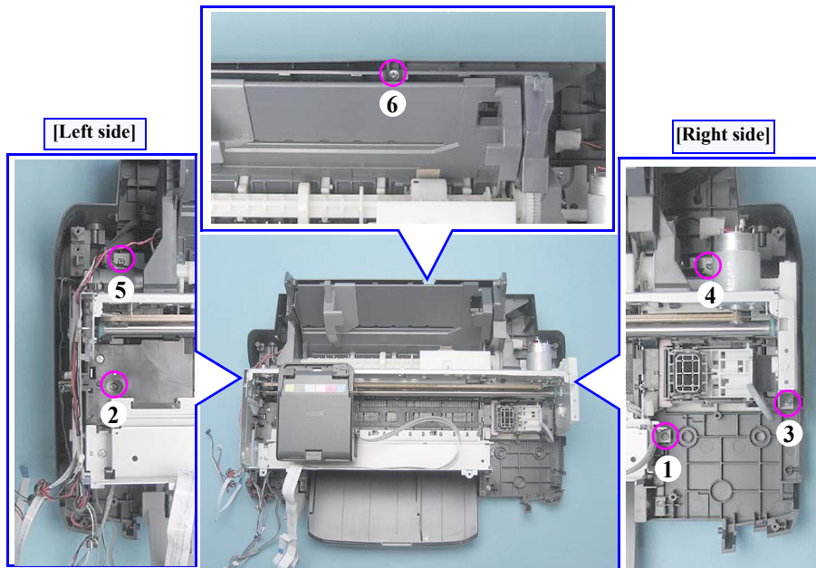
Figure 4-86. Removing the Screws (Printer Mechanism)
