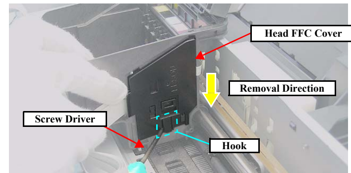
Figure 4-95. Removing the Head FFC Cover
