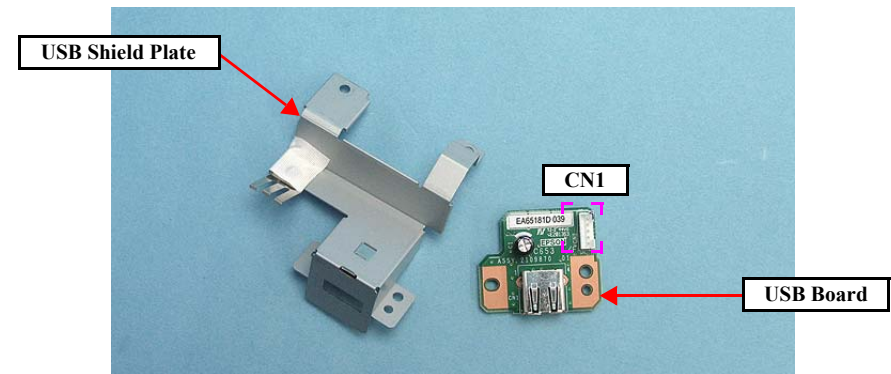
Figure 4-45. Disassembling the USB Board
