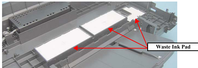
Figure 4-104. Removing the Waste Ink Pad
