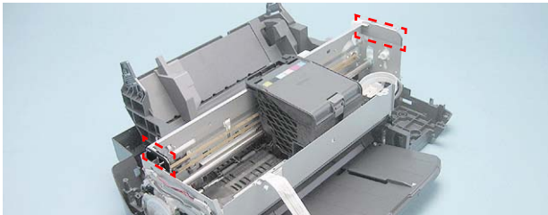
Figure 4-82. Handling the Printer Mechanism
