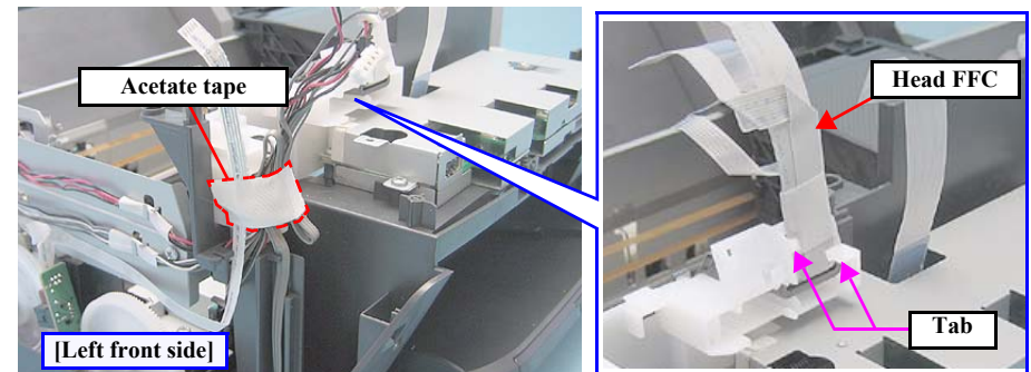
Figure 4-46. Removing the Cables
