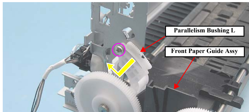
Figure 4-156. Removing the Parallelism Bushing L
