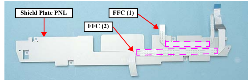
Figure 4-73. Removing the FFC
