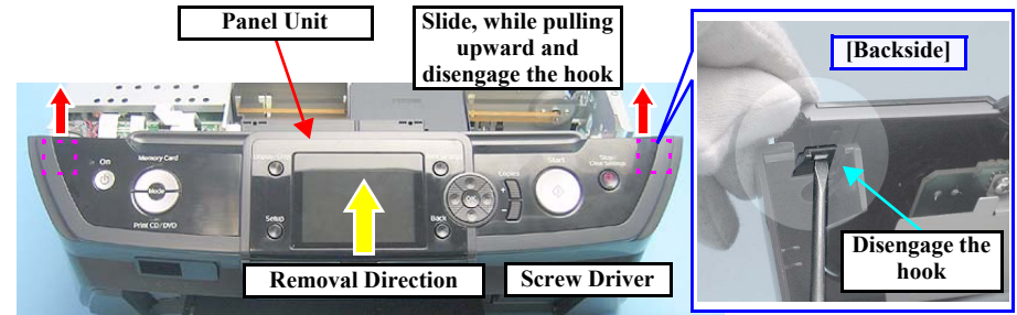
Figure 4-24. Removing the Panel Unit
