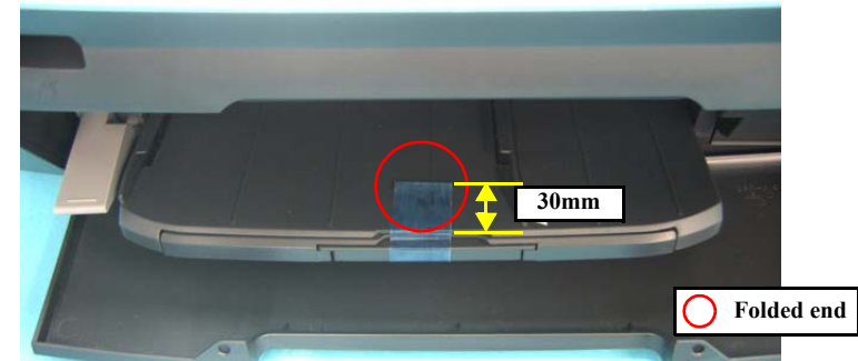
Figure 4-4. Securing the Stacker
