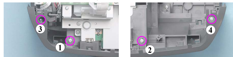
Figure 4-36. Removing the Front Housing (1)
