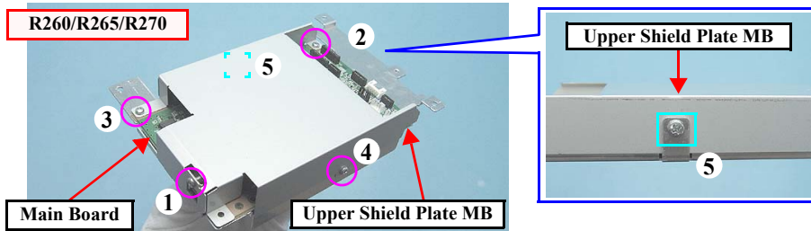
Figure 4-62. Removing the Upper Shield Plate MB (R260/R265/R270)
