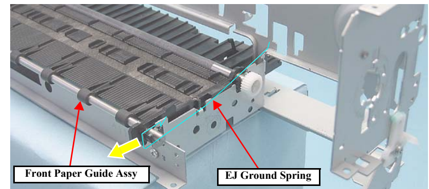
Figure 4-158. Removing the EJ Ground Spring
