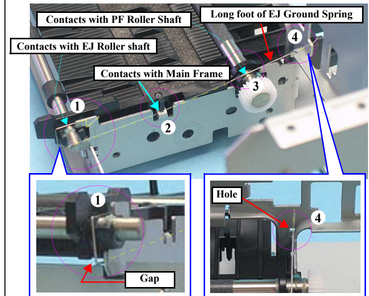
Figure 4-162. Attaching the EJ Ground Spring
