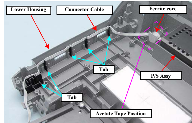
Figure 4-106. Removing the Connector Cables of the P/S Assy
