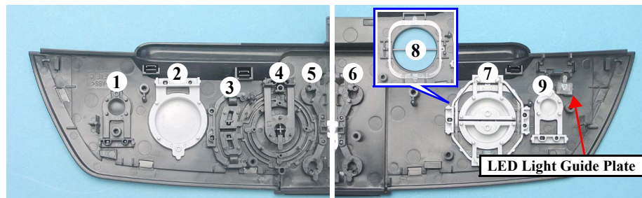
Figure 4-72. Removing the SW Buttons
