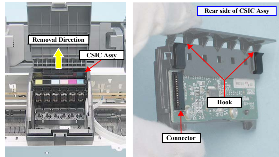
Figure 4-100. Removing the CSIC Assy (3)
