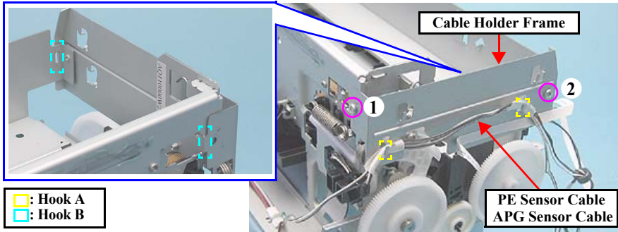
Figure 4-128. Removing the Cable Holder Frame
