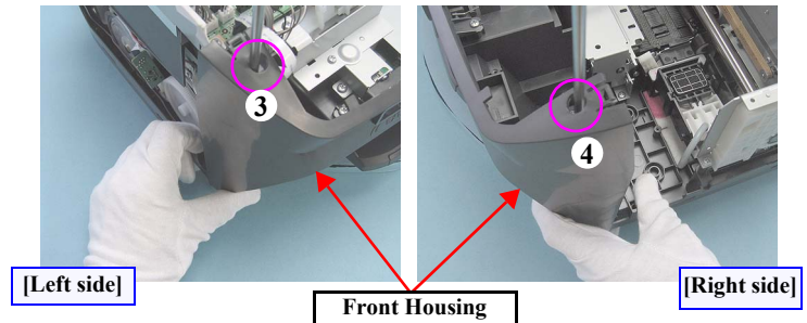
Figure 4-42. Reinstalling the Front Housing (3)
