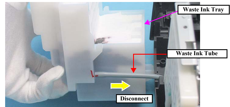
Figure 4-31. Removing the Waste Ink Tray (2)
