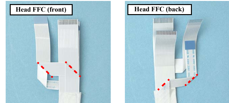
Figure 4-50. Routing the Head FFC (2)
