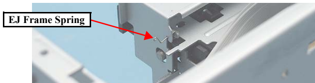
Figure 4-28. Cautions on removing the Waste Ink Tray
