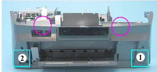
Figure 4-40. Reinstalling the Front Housing (1)
