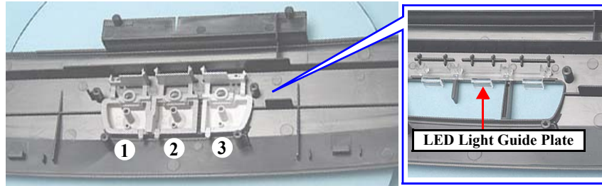
Figure 4-76. Removing the SW Buttons (R260/R265/R270)
