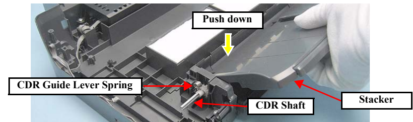
Figure 4-109. Removing the CDR Guide Lever Spring (1)
