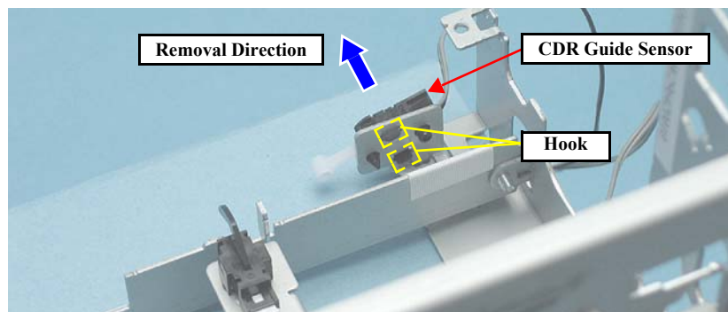
Figure 4-164. Removing the CDR Guide Sensor
