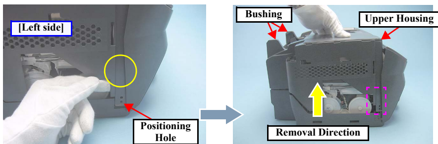
Figure 4-22. Removing the Upper Housing (2)
