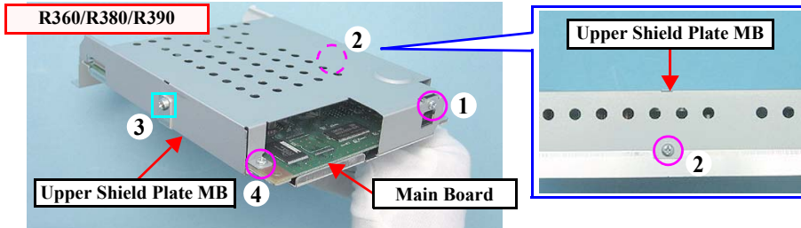
Figure 4-61. Removing the Upper Shield Plate MB (R360/R380/R390)
