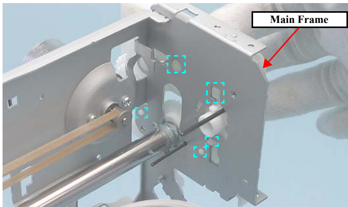
Figure 4-94. Reinstalling the APG Unit (4)
