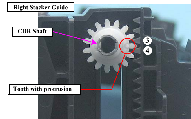
Figure 4-113. Reinstalling the CDR Shaft
