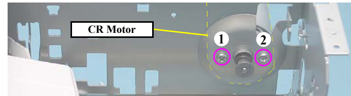
Figure 4-124. Removing the CR Motor (3)
