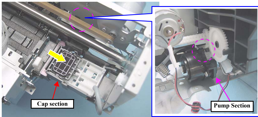
Figure 4-117. Removing the Ink System (2)
