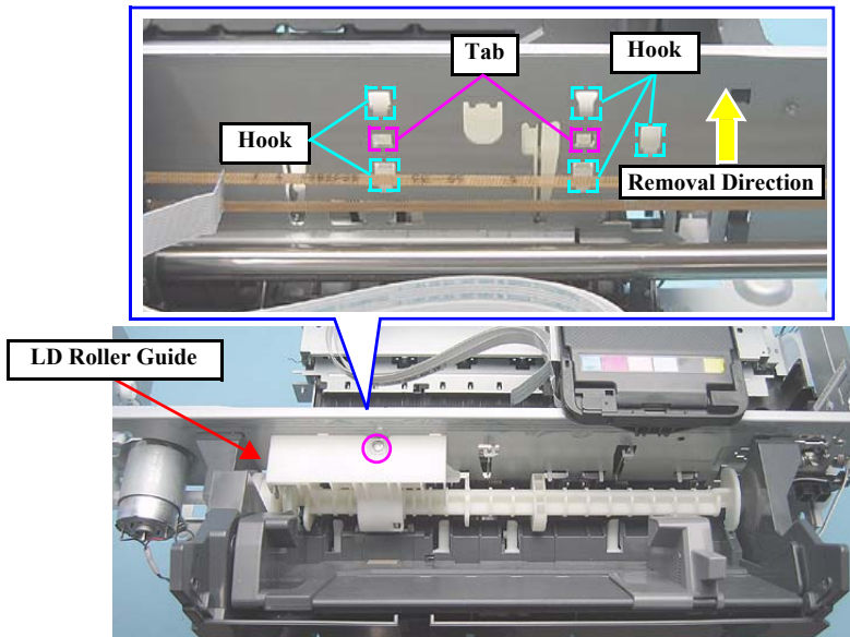
Figure 4-139. Removing the LD Roller Guide (1)
