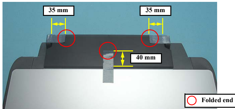
Figure 4-2. Securing the Paper Support
