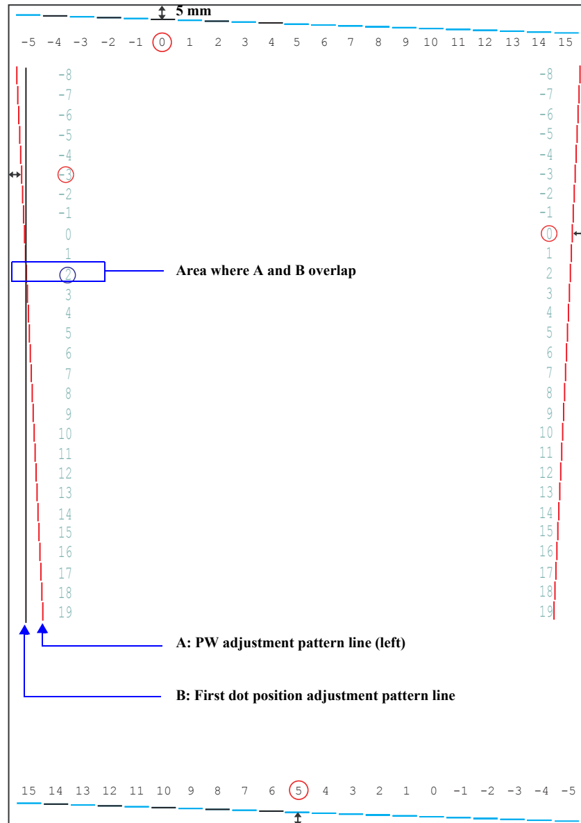
Figure 5-5. Left Right margin adjustment Pattern Printing
