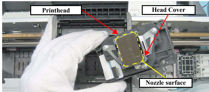
Figure 4-101. Handling of the Printhead
