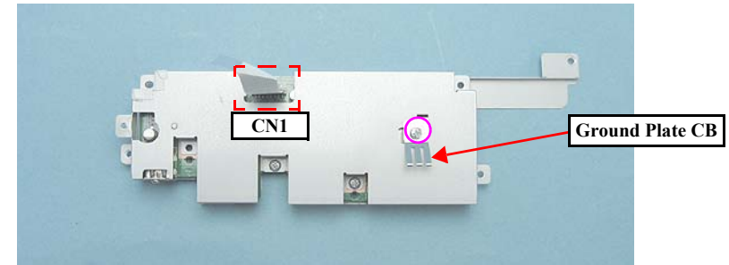
Figure 4-65. Card Board Disassembly
