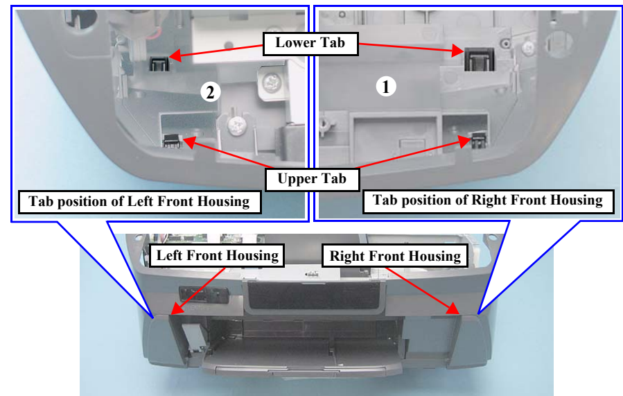
Figure 4-33. Removing Left/Right Front Housings (1)
