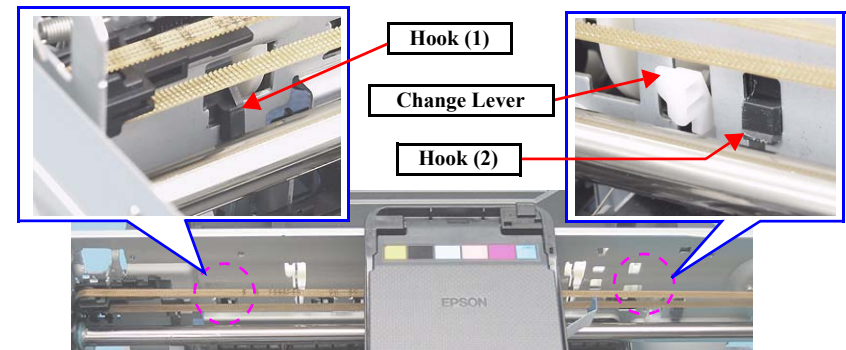
Figure 4-142. Disengaging the Hooks (ASF Unit)
