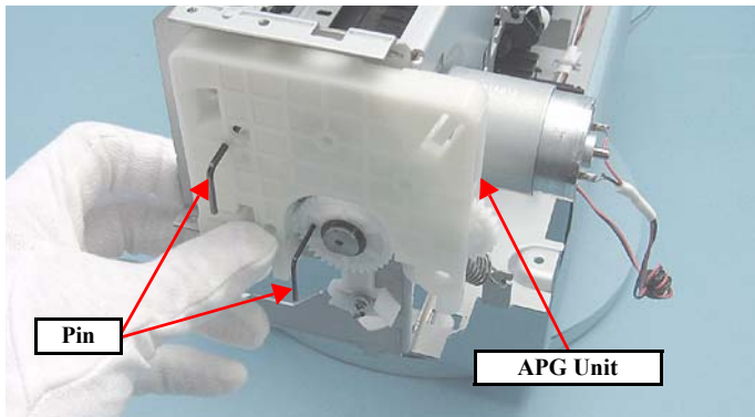
Figure 4-93. Reinstalling the APG Unit (3)
