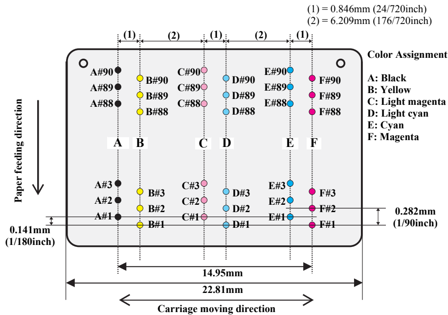
Figure 1-2. Nozzle Configuration
