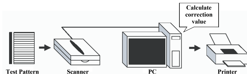
Figure 5-11. System Configuration
