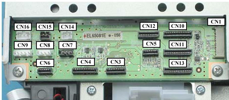
Figure 4-52. R360/R380/R390 Main Board
