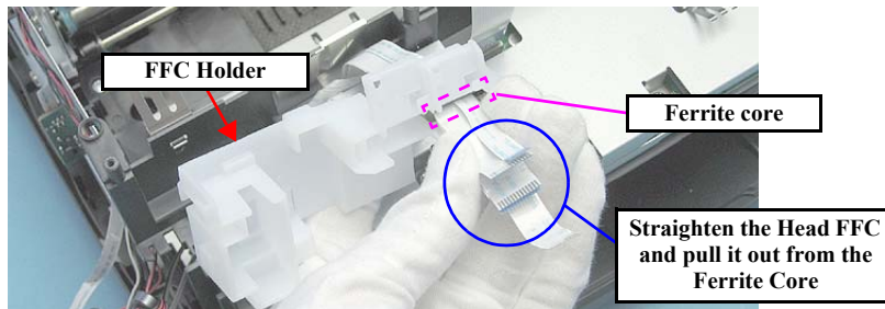
Figure 4-48. Removing the FFC Holder (2)
