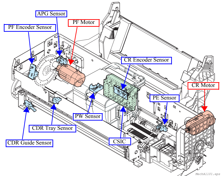
Figure 2-2. Motors & Sensors in the Printer Mechanism
