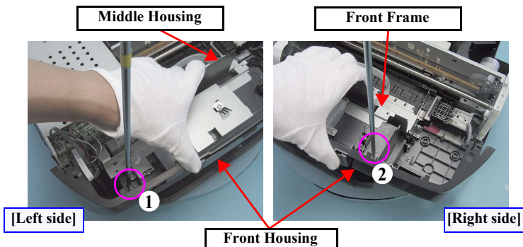
Figure 4-41. Reinstalling the Front Housing (2)
