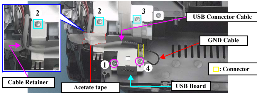
Figure 4-44. Removing the USB Board
