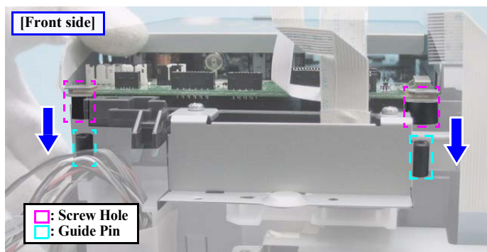
Figure 4-58. Reinstalling the Main Board Unit (2)
