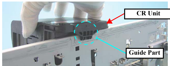
Figure 4-152. Reinstalling the CR Unit
