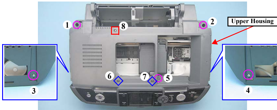
Figure 4-21. Removing the Upper Housing (1)
