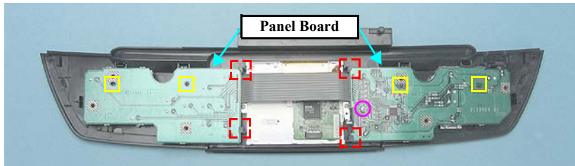
Figure 4-70. Removing the Panel Board (3)
