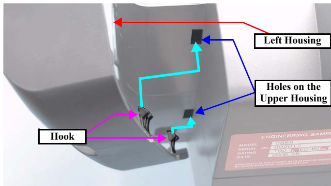
Figure 4-19. Reinstalling the Right/Left Housings
