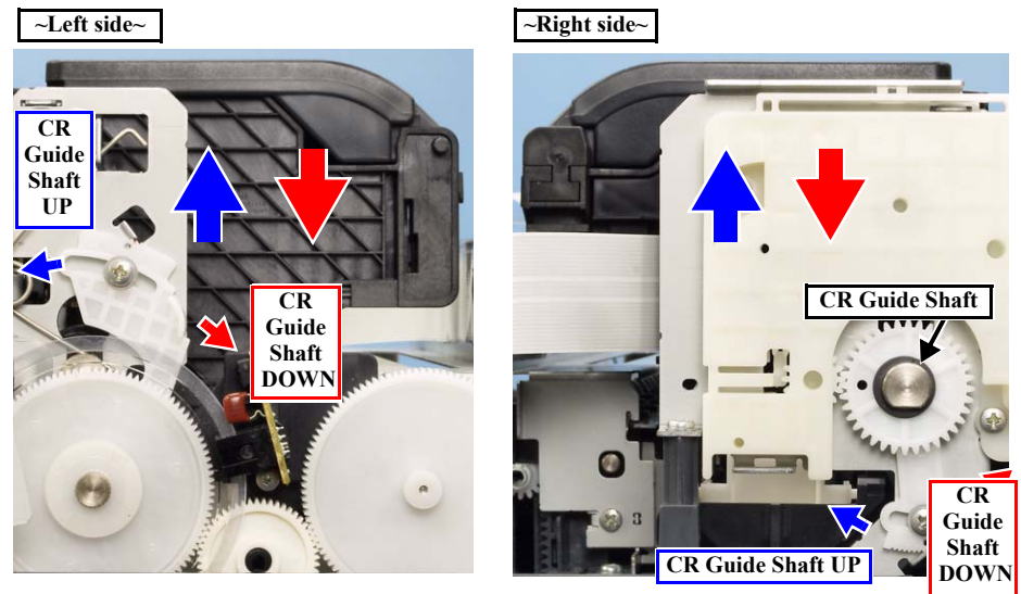
Figure 5-10. PG Adjustment 2
