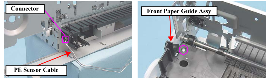
Figure 4-157. Removing the PE Sensor Cable
