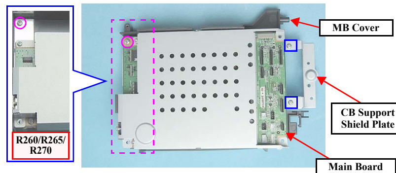
Figure 4-60. Removing the MB Cover/CB Shield Plate Support
