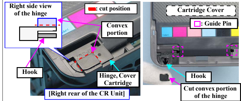
Figure 4-153. Removing the Cartridge Cover
