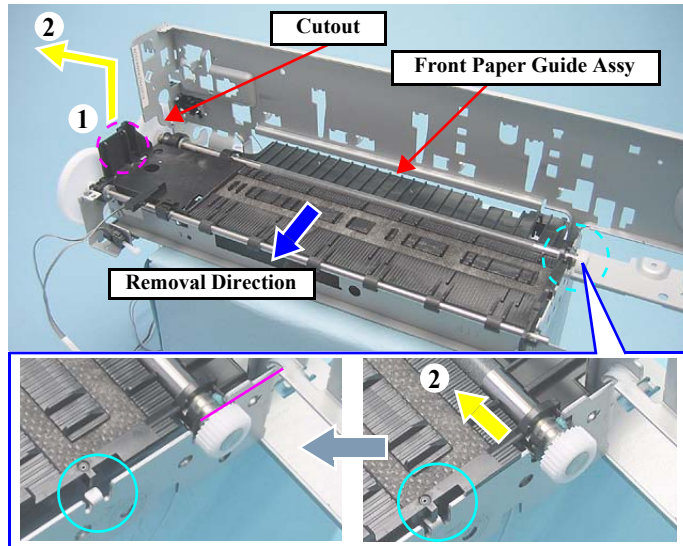
Figure 4-159. Removing the Front Paper Guide Assy
