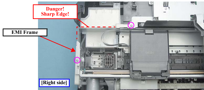
Figure 4-26. Removing the EMI Frame
