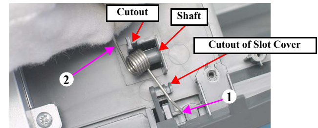
Figure 4-43. Reinstalling the Torsion Spring (R360/R380/R390 only)
