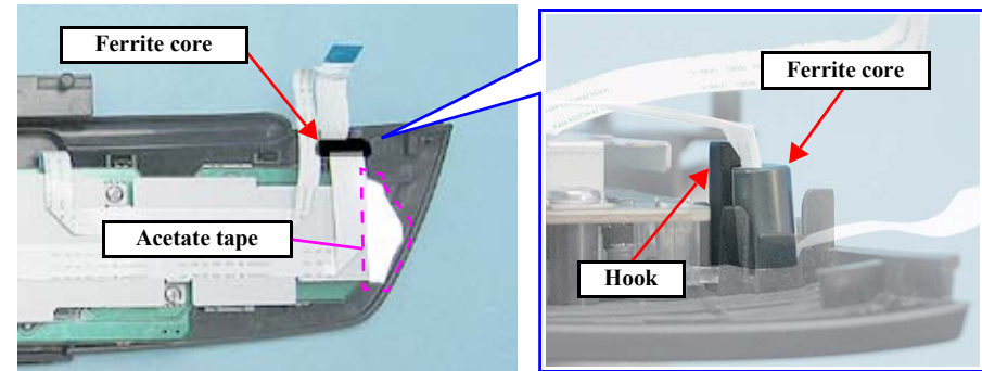
Figure 4-68. Removing the Panel Board (1)
