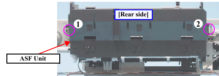
Figure 4-141. Removing the Screws (ASF Unit)
