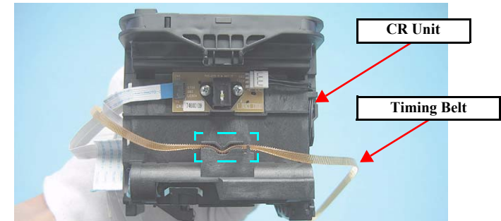
Figure 4-149. Removing the CR Unit (5)
