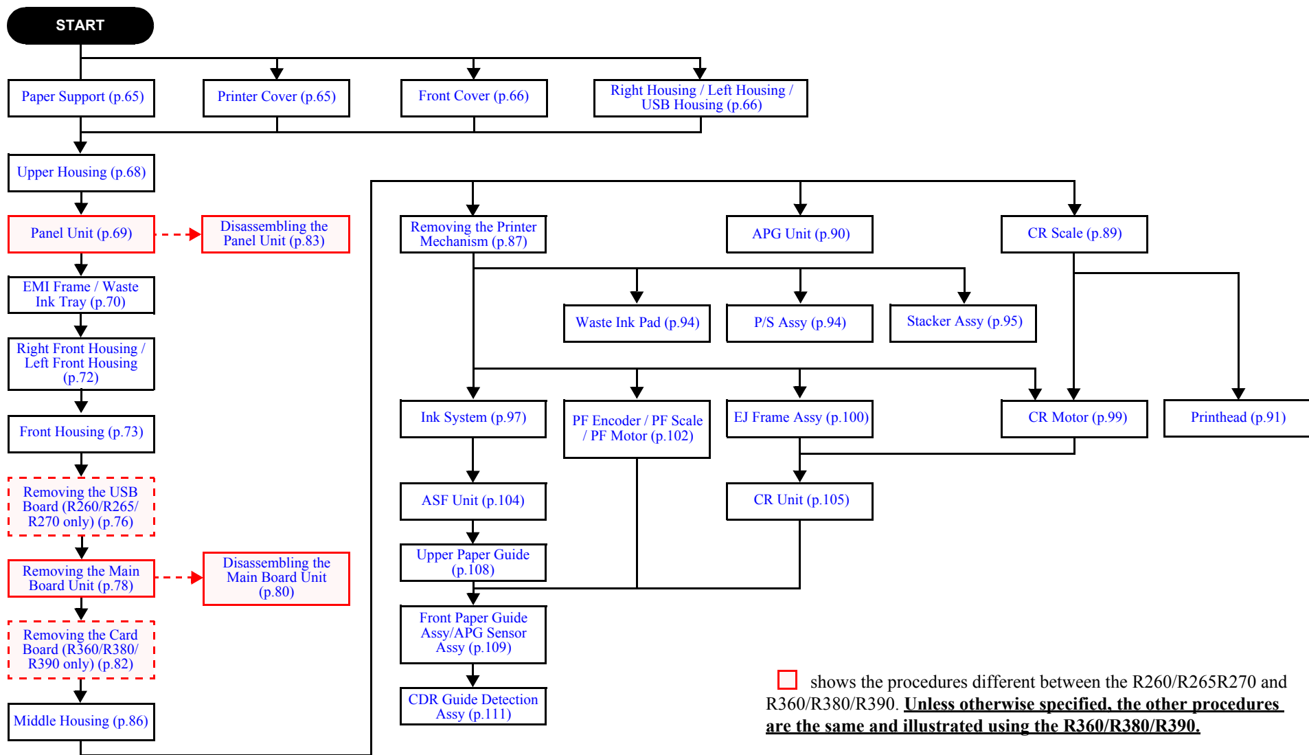
Flowchart 4-1. R260/R265/R270 & R360/R380/R390 Disassembly Flowchart
