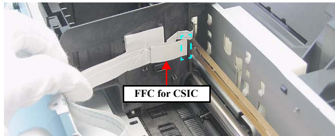
Figure 4-96. Removing the FFC for CSIC
