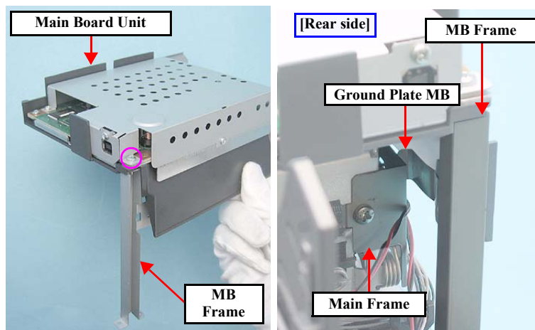
Figure 4-57. Reinstalling the Main Board Unit(1)
