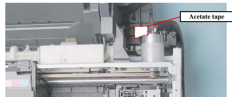
Figure 4-85. Removing the Ferrite Core (Printer mechanism)
