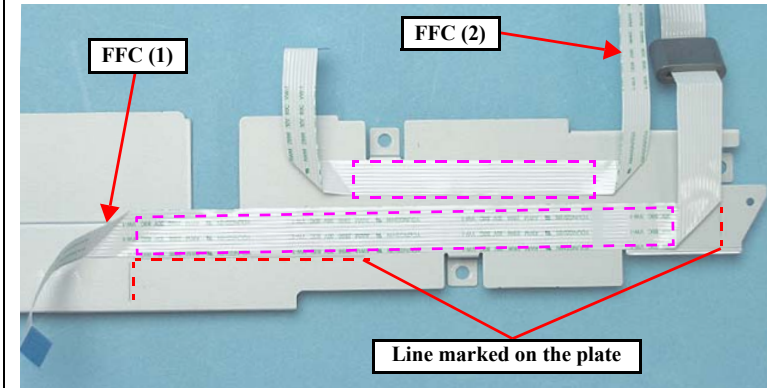
Figure 4-78. Attaching the FFC (1), FFC (2) (R360/R380/R390)
