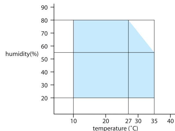
Figure 1-6. Temperature/Humidity Range
