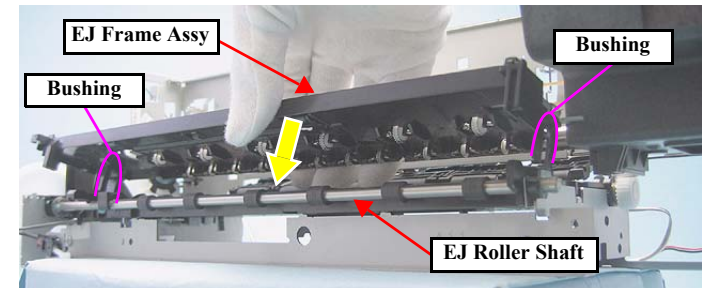
Figure 4-131. Reinstalling the EJ Frame Assy
