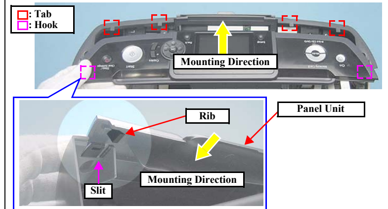
Figure 4-25. Reinstalling the Panel Unit
