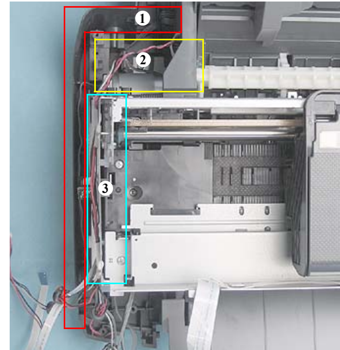
Figure 4-87. Routing the cables prior to Printer Mechanism installation
