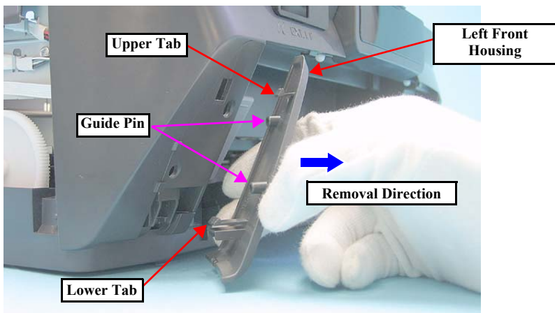
Figure 4-34. Tabs of the Right/Left Front Housings
