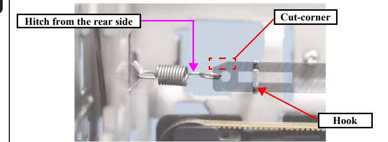
Figure 4-89. Reinstalling the CR Scale
