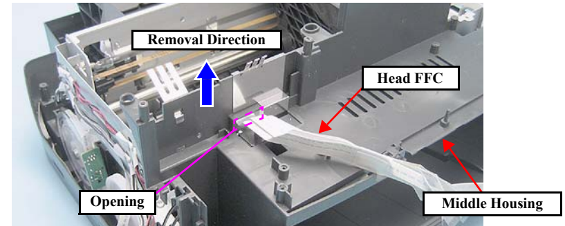
Figure 4-80. Removing the Middle Housing (2)
