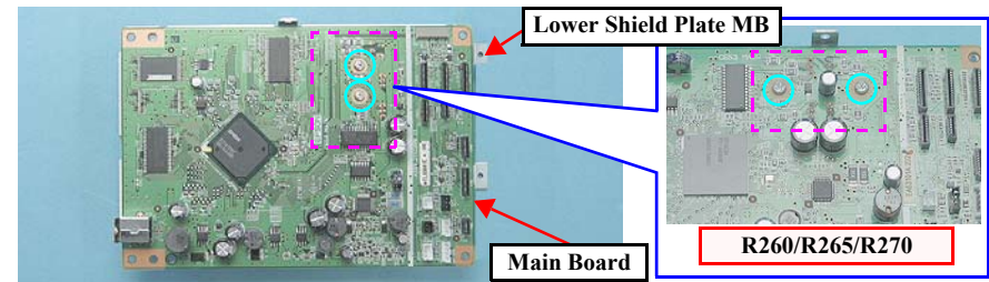
Figure 4-63. Removing the Main Board
