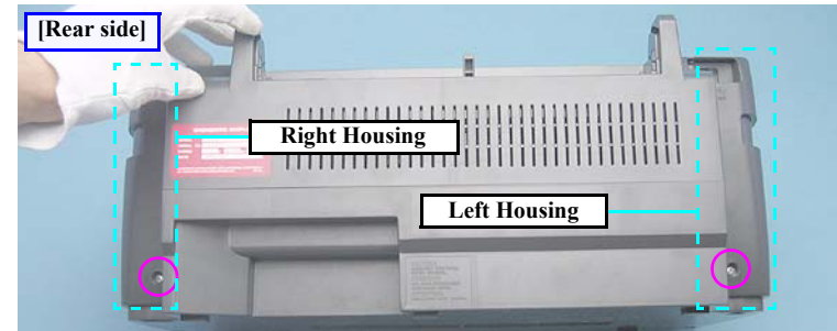
Figure 4-16. Removing the Right/Left Housings (1)
