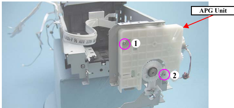
Figure 4-90. Removing the APG Unit
