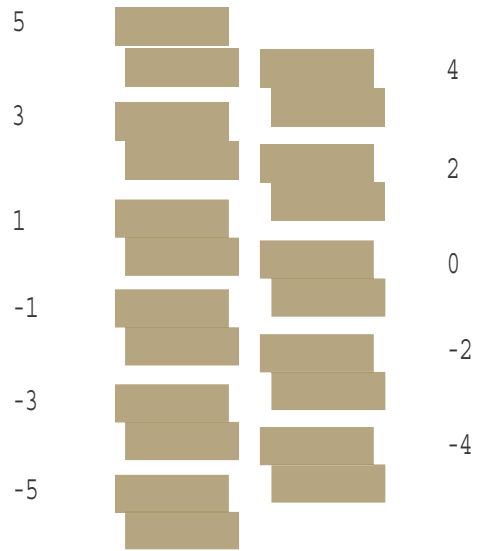
Figure 5-6. PF adjustment (Standard Area) Pattern Printing
