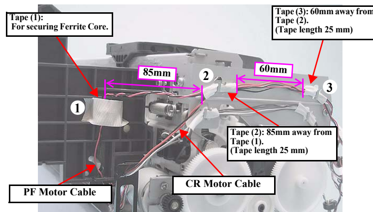
Figure 4-138. Routing/Securing the PF Motor/CR Motor Cables
