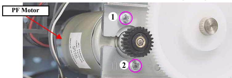
Figure 4-137. Removing the PF Motor
