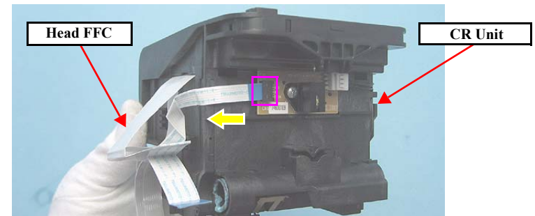
Figure 4-150. Removing the CR Unit (6)
