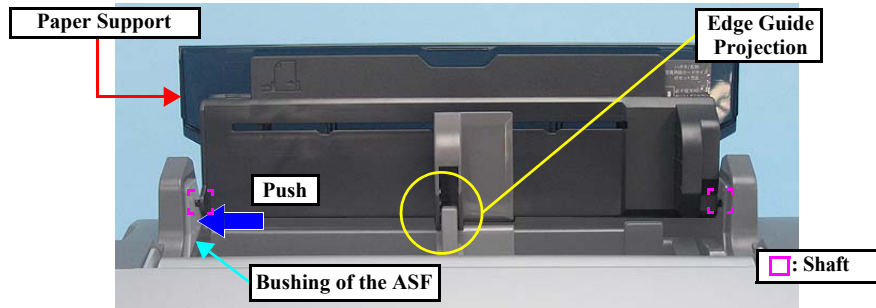
Figure 4-11. Removing the Paper Support
