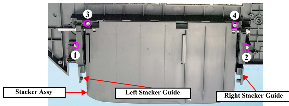
Figure 4-111. Removing the Stacker Assy
