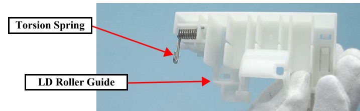
Figure 4-140. Removing the LD Roller Guide (2)
