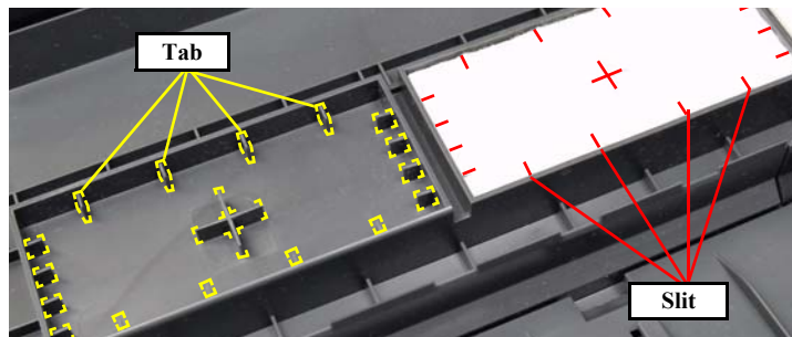
Figure 4-105. Reinstalling the Waste Ink Pads
