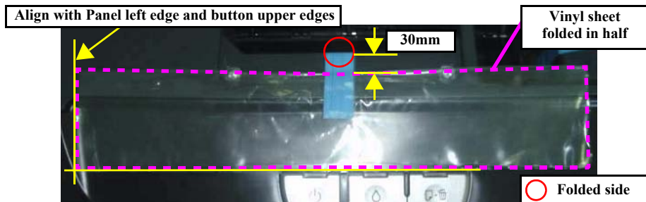
Figure 4-6. Protecting the Panel Unit (R260/R265/R270 only)
