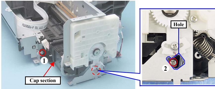
Figure 4-116. Removing the Ink System (1)
