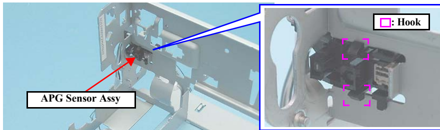
Figure 4-160. Removing the APG Sensor
