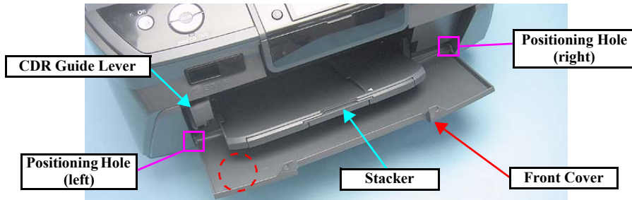
Figure 4-15. Removing the Front Cover (1)
