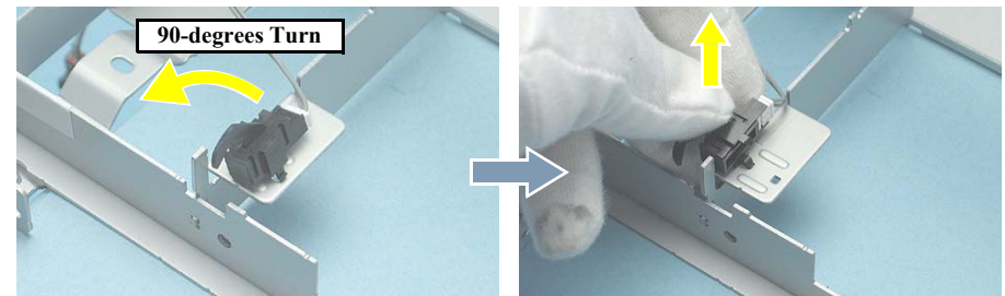
Figure 4-165. Removing the CDR Tray Sensor (CDR Guide Detection Assy)
