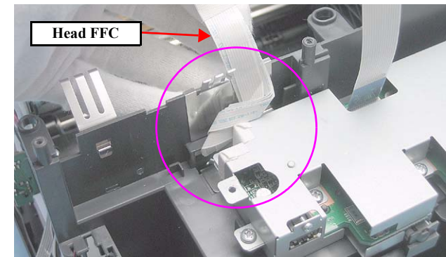
Figure 4-66. Routing the Head FFC (1)
