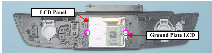
Figure 4-71. Removing the LCD Panel
