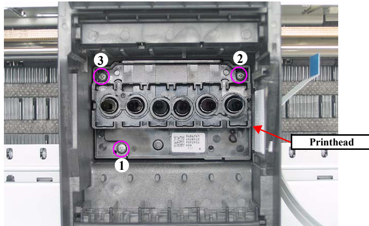
Figure 4-102. Removing the Printhead (1)
