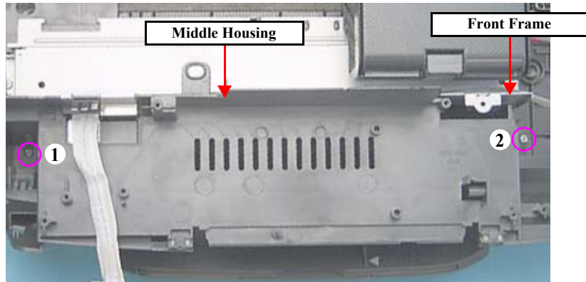
Figure 4-79. Removing the Middle Housing (1)
