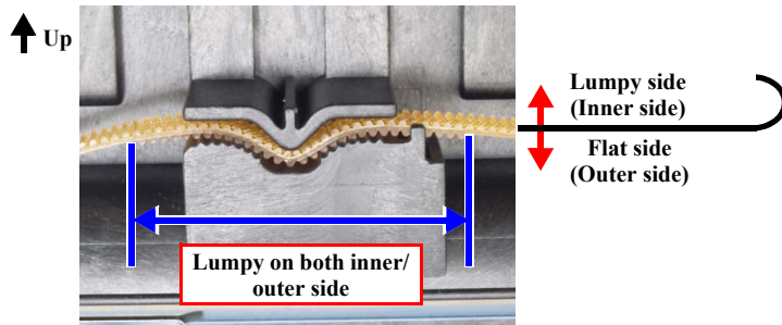
Figure 4-151. Reinstalling the Timing Belt
