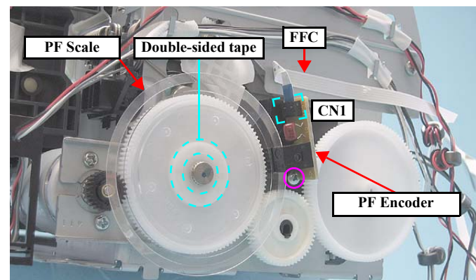
Figure 4-135. Removing the PF Encoder/PF Scale
