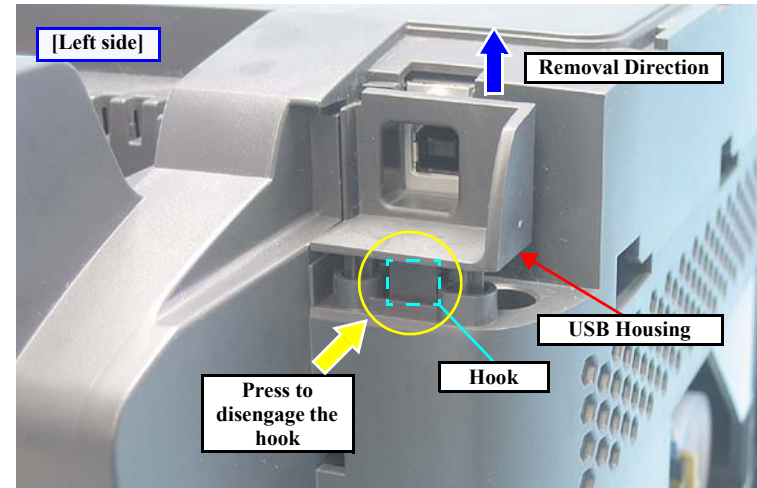
Figure 4-20. Removing the USB Housing
