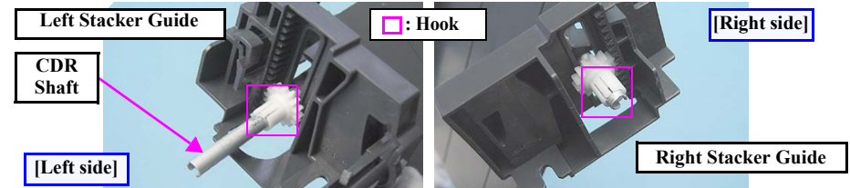
Figure 4-112. Removing the CDR Shaft
