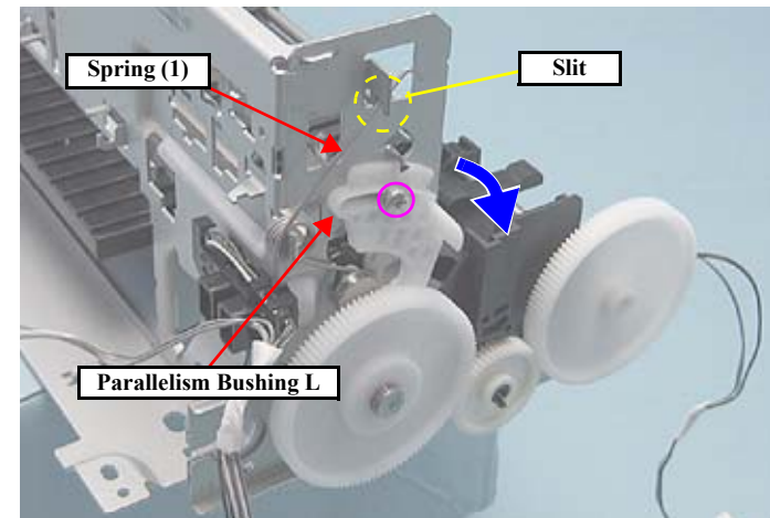
Figure 4-145. Removing the CR Unit (1)
