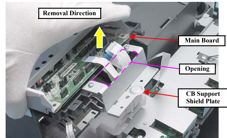
Figure 4-56. Removing the Main Board Unit (2)
