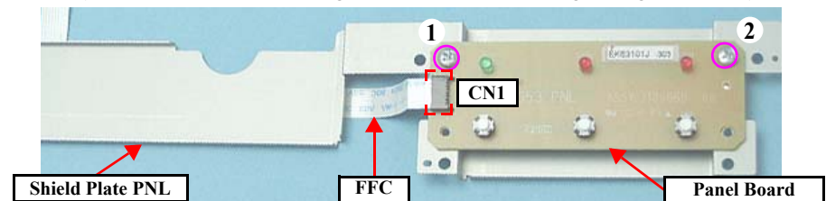
Figure 4-75. Removing the Panel Board (R260/R265/R270)
