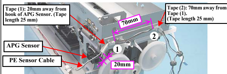
Figure 4-134. Acetate Tape Position
