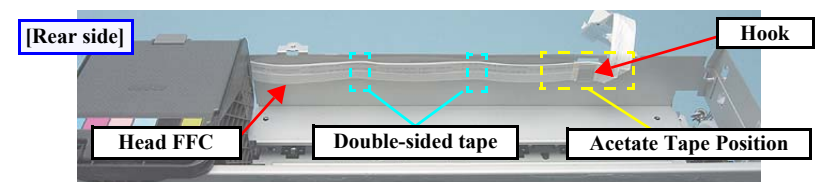
Figure 4-127. Removing the Head FFC
