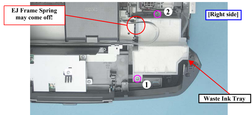
Figure 4-30. Removing the Waste Ink Tray (1)
