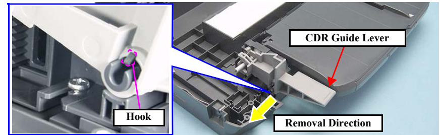
Figure 4-108. Removing the CDR Guide Lever
