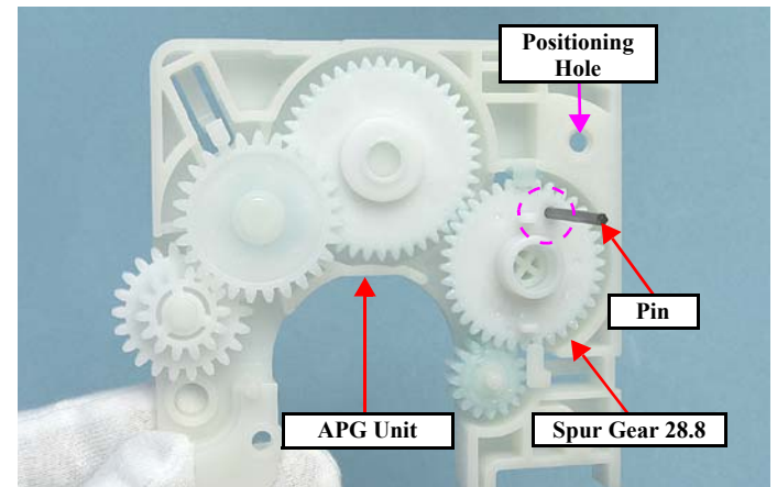
Figure 4-92. Reinstalling the APG Unit (2)
