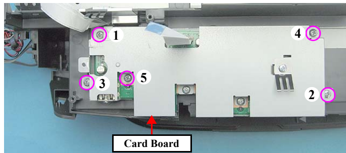
Figure 4-64. Removing the Card Board
