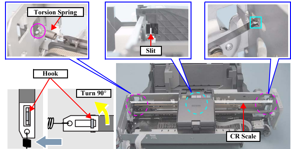
Figure 4-88. Removing the CR Scale
