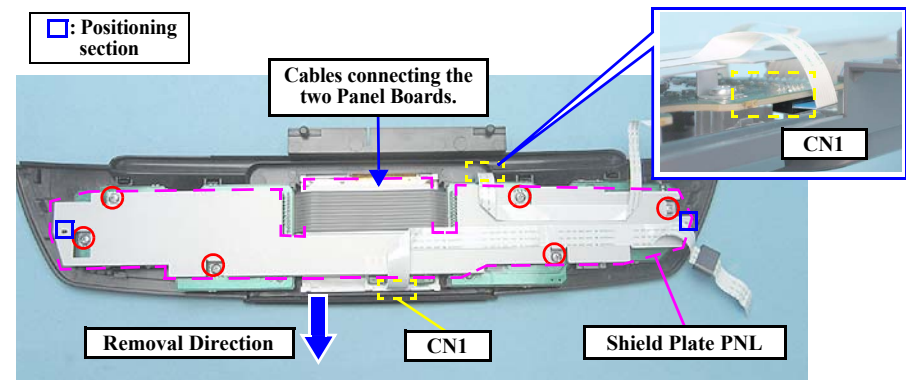
Figure 4-69. Removing the Panel Board (2)
