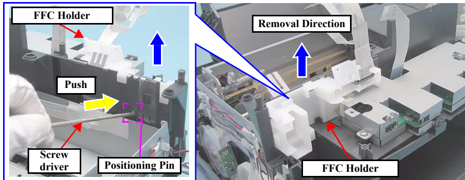
Figure 4-47. Removing the FFC Holder (1)
