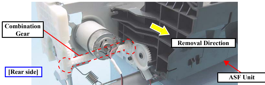
Figure 4-143. Removing the ASF Unit
