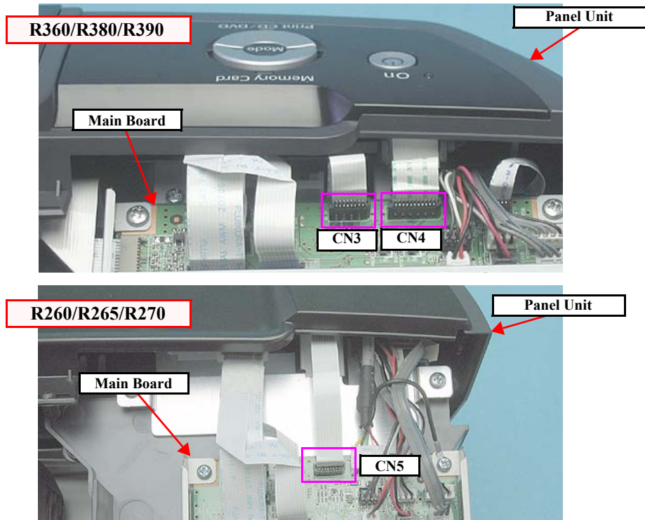
Figure 4-23. Removing the Connectors (Panel Unit)
