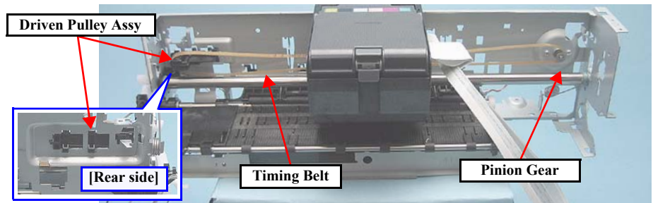
Figure 4-122. Removing the CR Motor (1)
