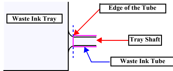
Figure 4-32. Cautions of installing the Waste Ink Tray
