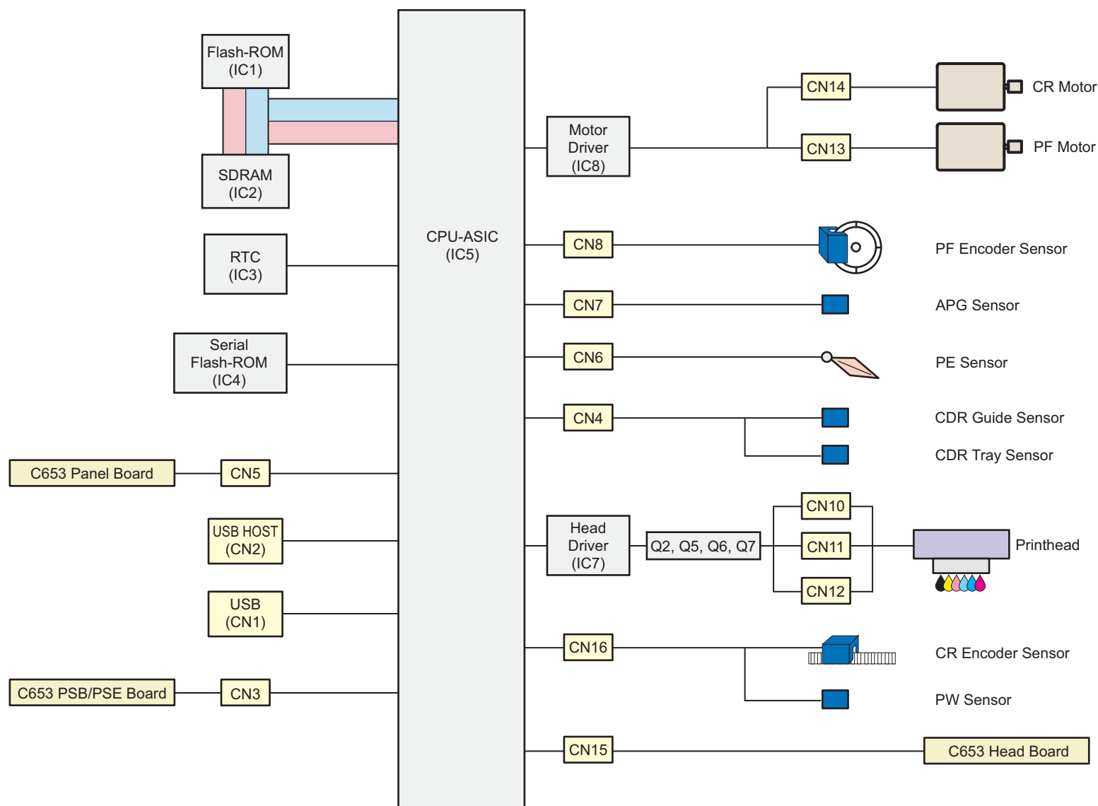
Figure 2-4. Circuit Block Diagram for R260/R265/R270
