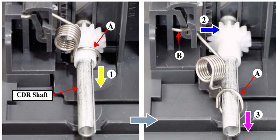
Figure 4-110. Removing the CDR Guide Lever Spring (2)
