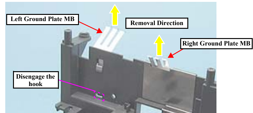
Figure 4-81. Removing the Middle Housing (3)
