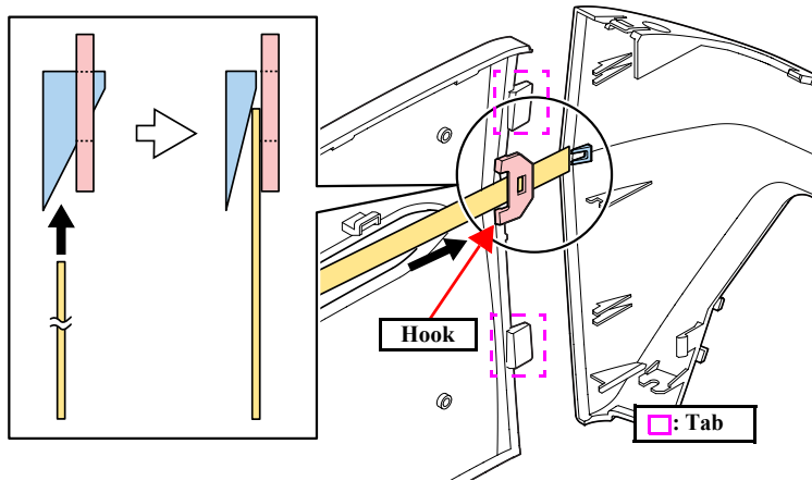
Figure 4-18. Disengaging the Hook and Tabs
