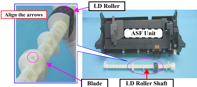
Figure 4-144. Reinstalling the LD Roller
