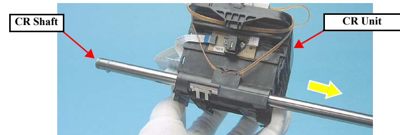
Figure 4-148. Removing the CR Unit (4)
