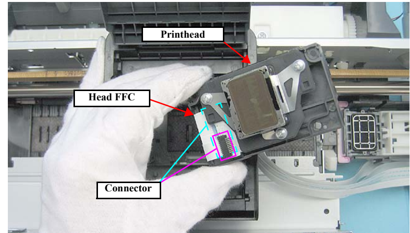
Figure 4-103. Removing the Printhead (2)
