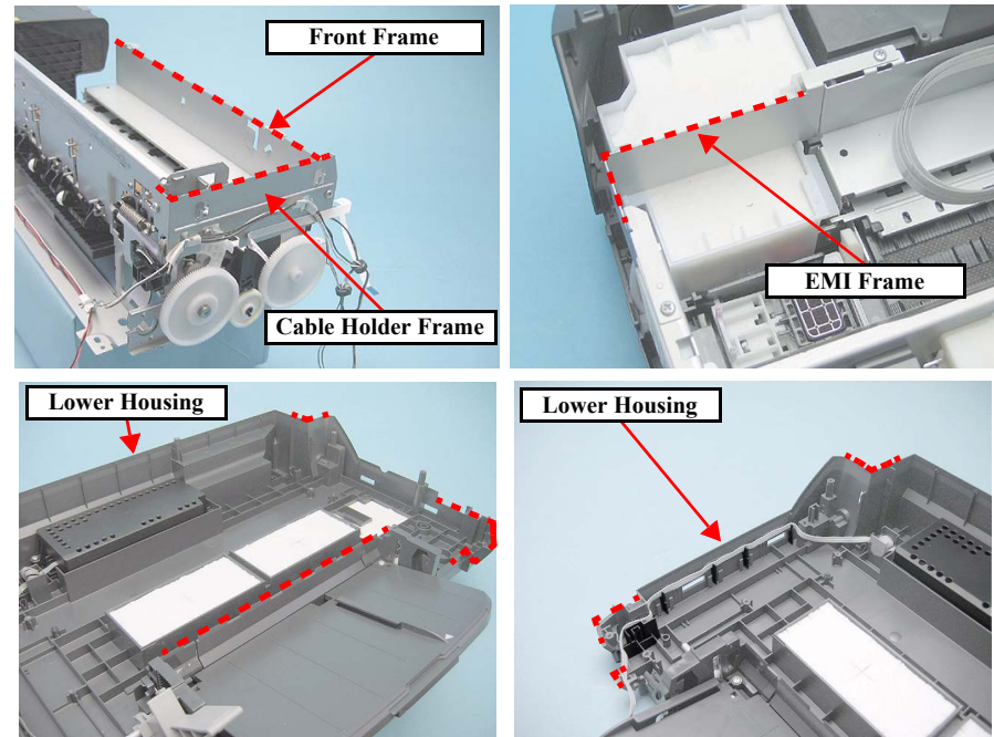
Figure 4-9. Sharp Metal Edges
