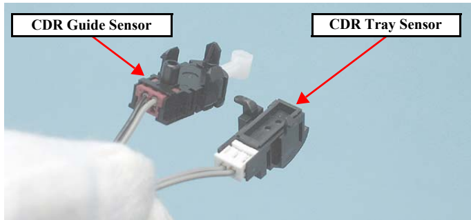
Figure 4-163. CDR Guide Detection Assy
