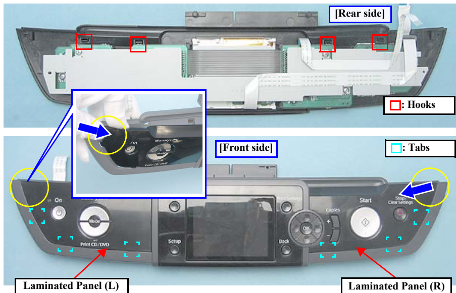
Figure 4-67. Removing the Left/Right Laminated Panels
