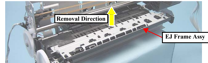
Figure 4-130. Removing the EJ Frame Assy
