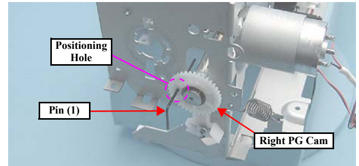
Figure 4-91. Reinstalling the APG Unit (1)
