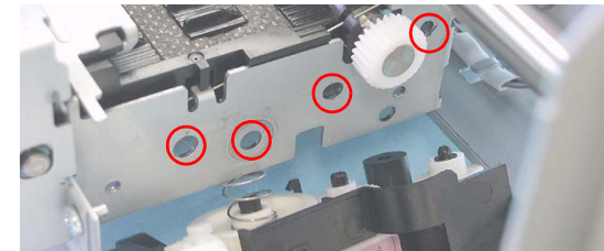
Figure 4-119. Reinstalling the Ink System (1)
