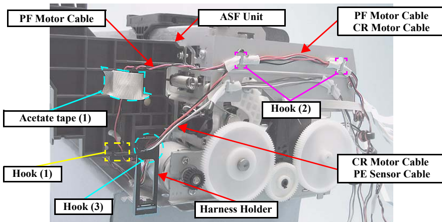
Figure 4-136. Removing the Harness Holder
