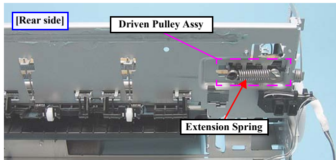
Figure 4-121. Removing the Extension Spring
