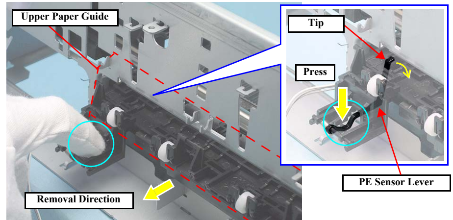
Figure 4-155. Removing the Upper Paper Guide (2)
