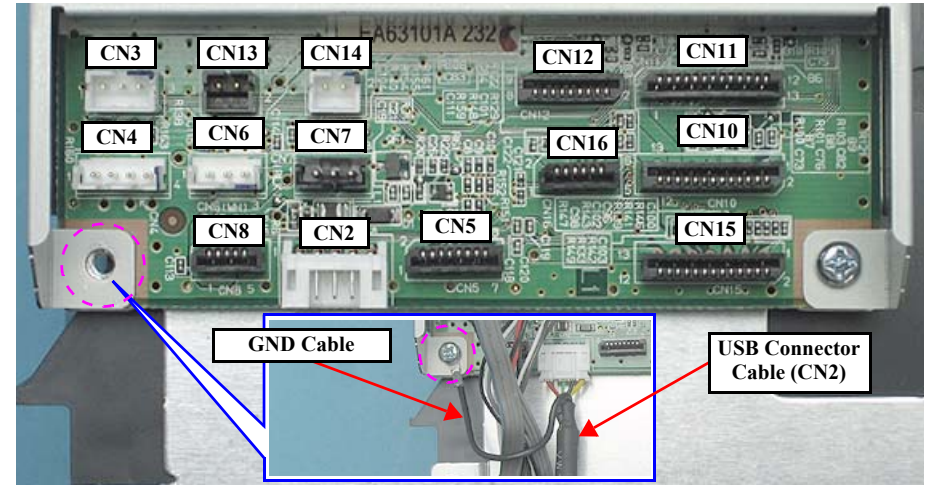
Figure 4-53. R260/R265/R270 Main Board
