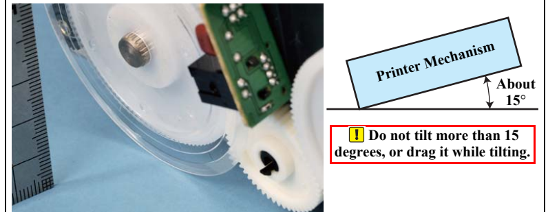
Figure 4-84. Handling of the Printer Mechanism
