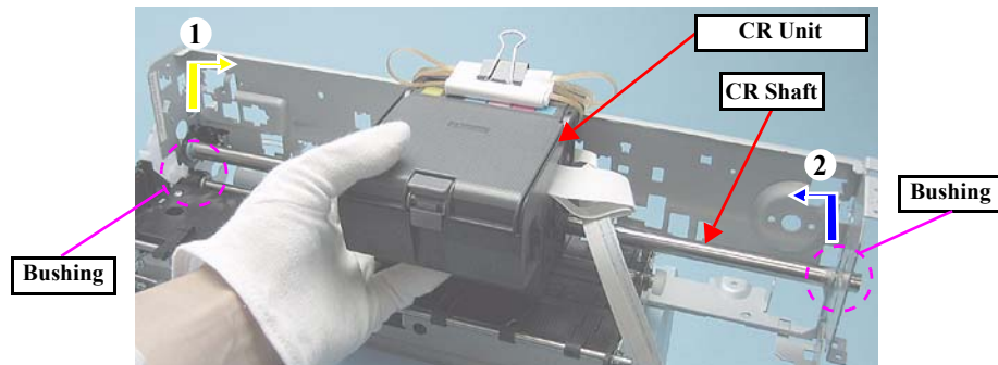
Figure 4-147. Removing the CR Unit (3)
