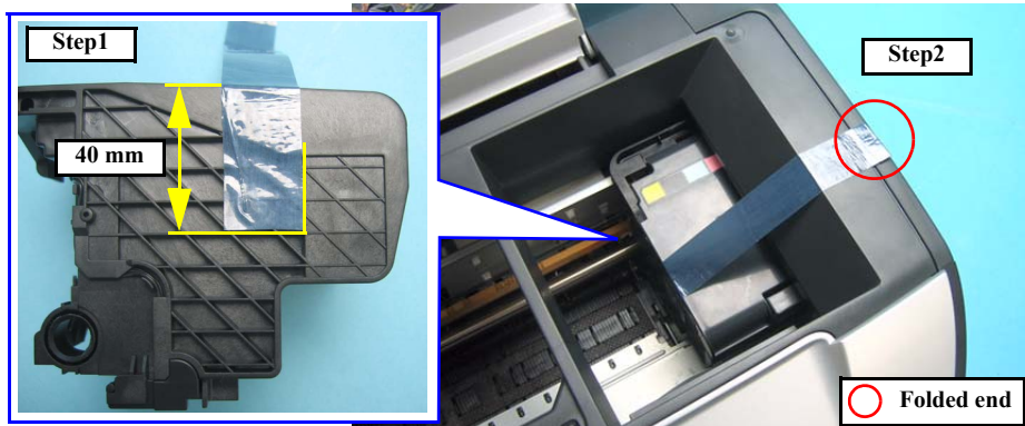
Figure 4-1. Securing the Carriage
