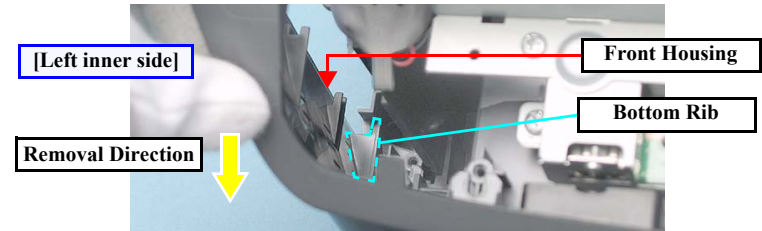
Figure 4-38. Caution as to Removing the Front Housing
