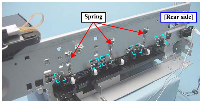
Figure 4-154. Removing the Upper Paper Guide (1)
