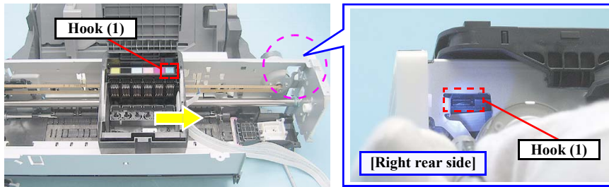
Figure 4-98. Removing the CSIC Assy (1)
