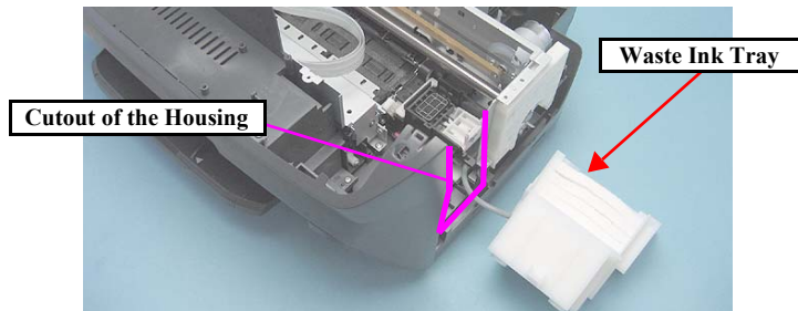
Figure 4-29. Handling of the Waste Ink Tray
