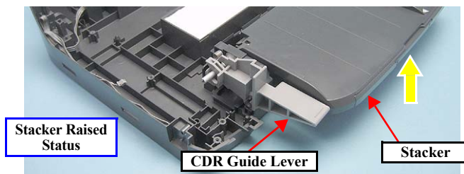
Figure 4-83. Cautions on Removing the Printer Mechanism
