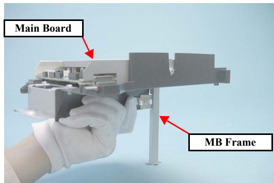
Figure 4-55. Cautions on Removing the Main Board Unit
