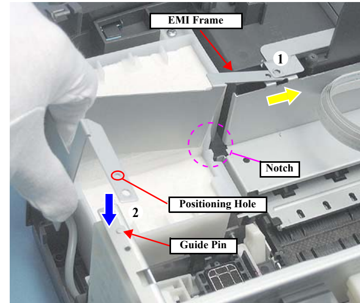
Figure 4-27. Reinstalling the EMI Frame
