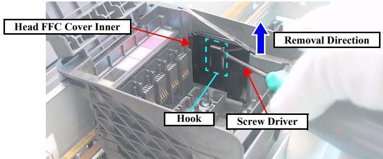
Figure 4-97. Removing the Head FFC Cover Inner
