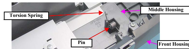
Figure 4-35. Removing the Torsion Spring (R360/R380/R390 only)
