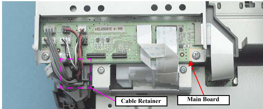
Figure 4-51. Removing the Cables (R360/R380/R390 Main Board)
