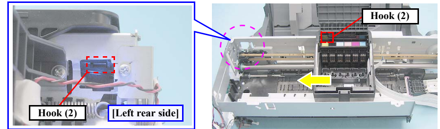
Figure 4-99. Removing the CSIC Assy (2)
