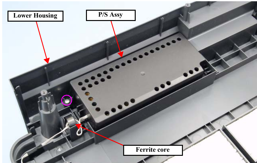
Figure 4-107. Removing the P/S Assy
