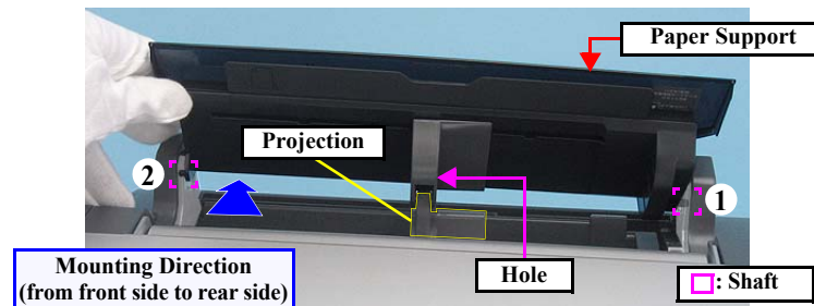
Figure 4-12. Reinstalling the Paper Support
