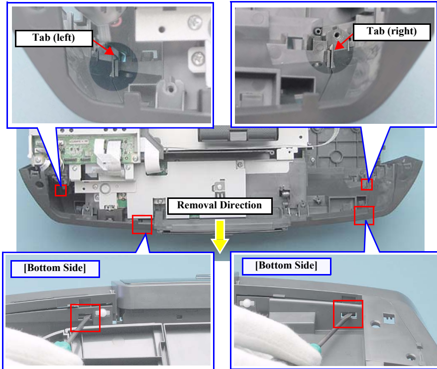
Figure 4-37. Removing the Front Housing (2)
