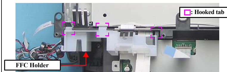
Figure 4-49. Reinstalling the FFC Holder
