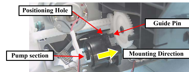
Figure 4-120. Reinstalling the Ink System (2)
